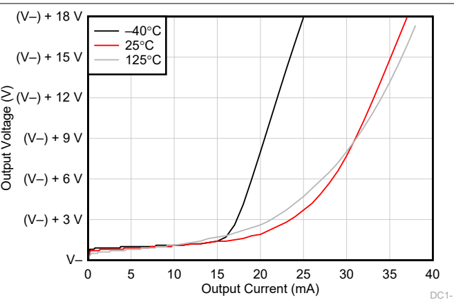
Figure 7-12. Output Voltage Swing vs Output Current (Sinking)
